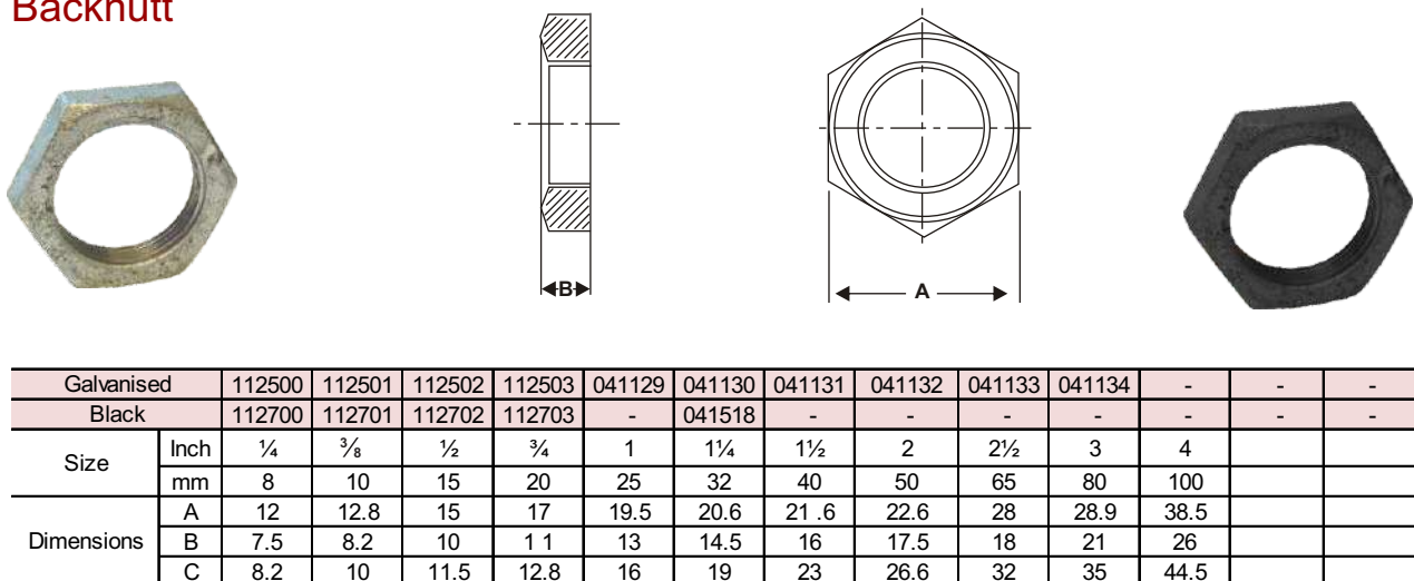
Fig 310 Backnutt
