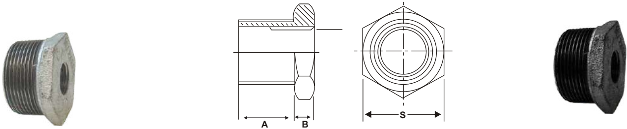
Fig 241 Bushes
