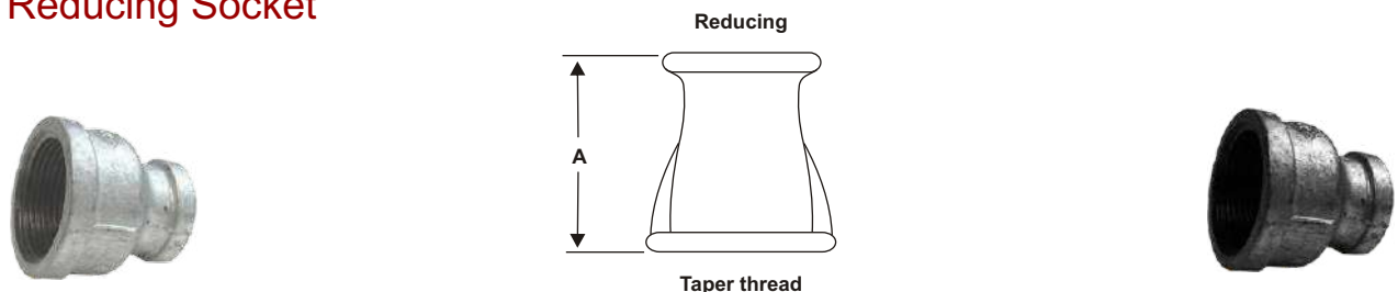
Fig 240 Reducing Socket
