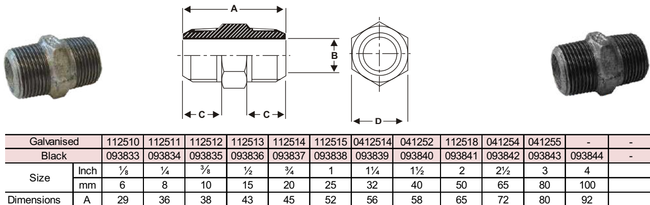
Fig 280 Hexagon Nipple
