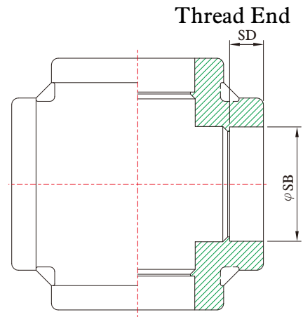
Socket-Weld End
